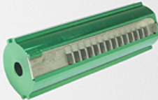
SDJA33 - Half Teeth Aluminum Piston w/ Removeable Steel Teeth
